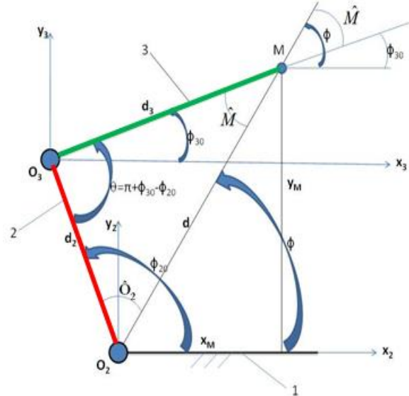
Fig. 3. Kinematic diagram of the kinematic chain plan 2-3 linked to item 1 considered fixed
