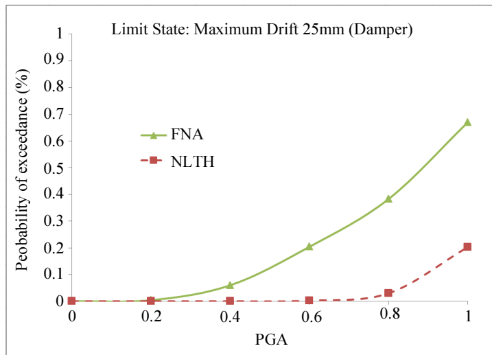
Fig. 7: Fragility curve for the RC frame supported by dampers
