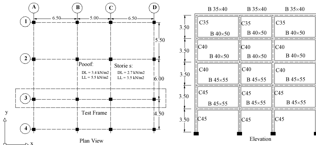
Fig. 2: Schematic plan view and elevation of the selected RC frame and loading amounts (kN, m)
