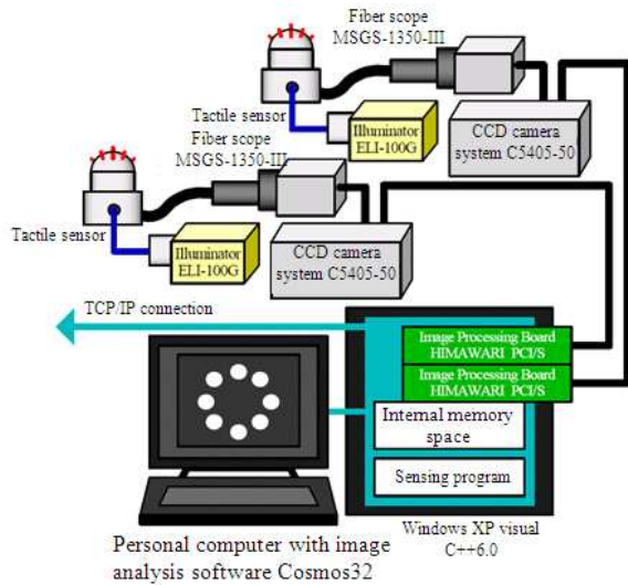
Fig. 3: Control system layout of optical three-axis tactile sensor
