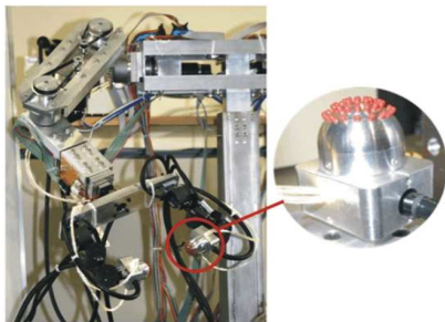
Fig. 1: Robot arm mounted with optical three-axis tactile sensors
