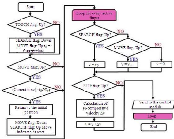
Fig. 8: Algorithm of robot hand speed estimator
