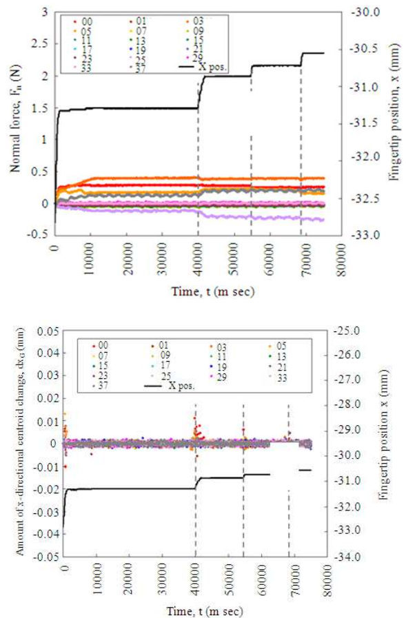
Fig. 6: Experiment of grasping paper cup with water. (Top) Experiment condition. (Middle) Normal force detection and right hand tip position at x-axis. (Bottom) Shear force detection and right hand tip position at x-axis
