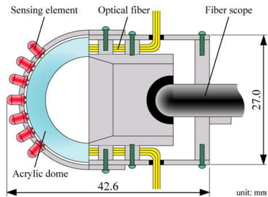
Fig. 2: Hardware structure of optical three-axis tactile sensor
