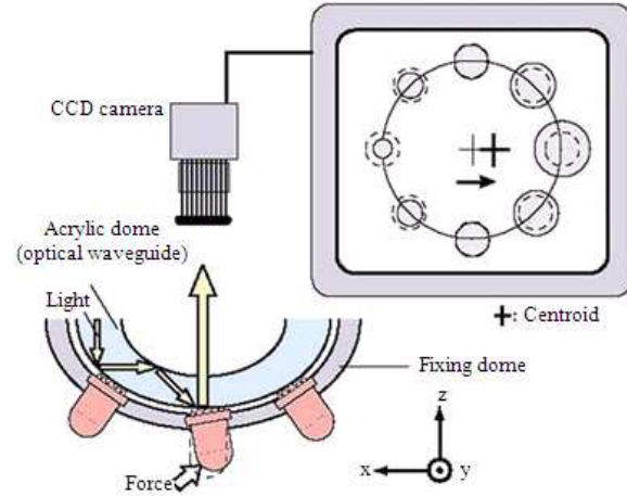
Fig. 5: Sensing principle of shear force detection
