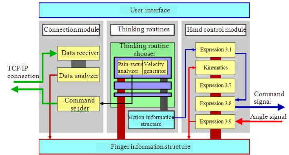
Fig. 4: Control system structure of robot hand
