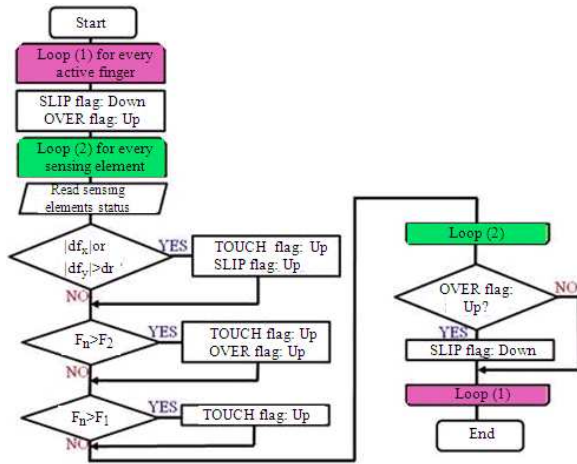
Fig. 7: Algorithm of flag analyzer in the robot control system
